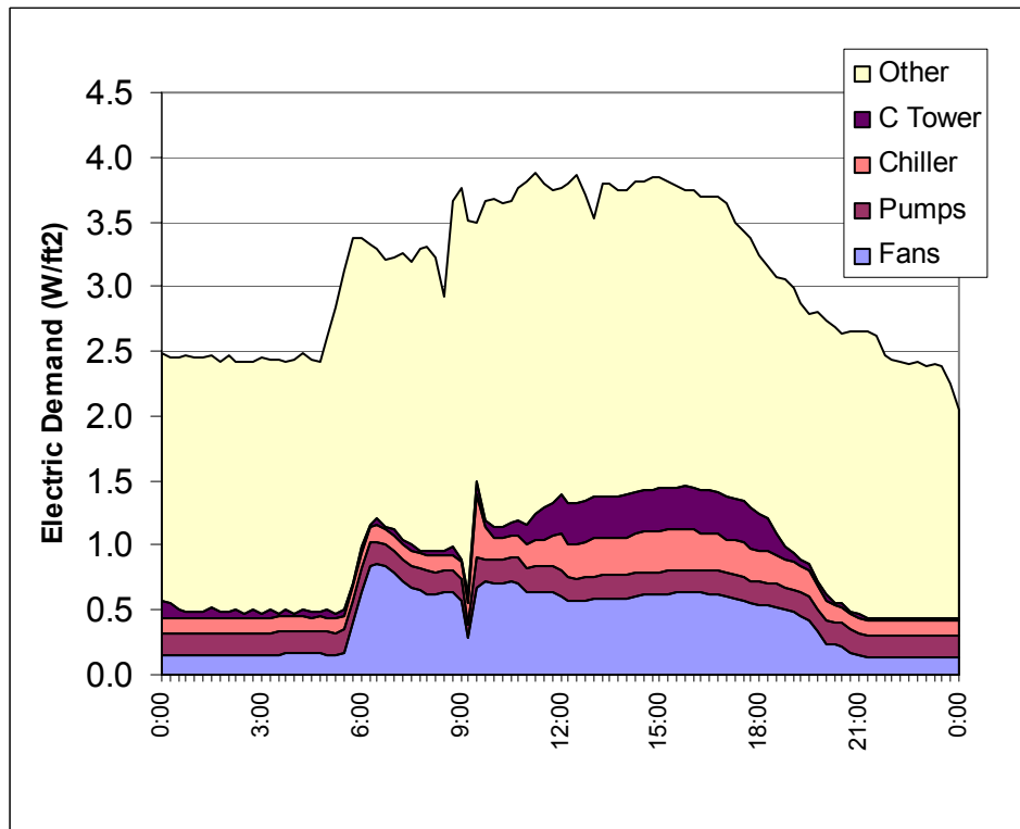
Figure 113. Peak Day Electric Demand, Site 1, 9/3/2002 (Cumulative Graph; Total Peak is 3.9 W/ft 2 )
