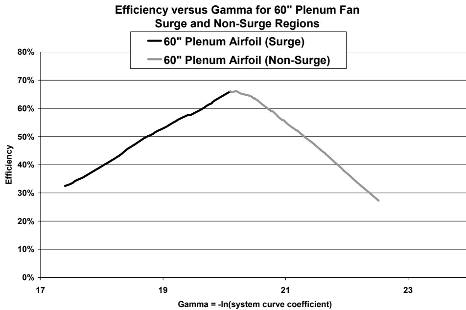
Figure 44. Gamma Curve
