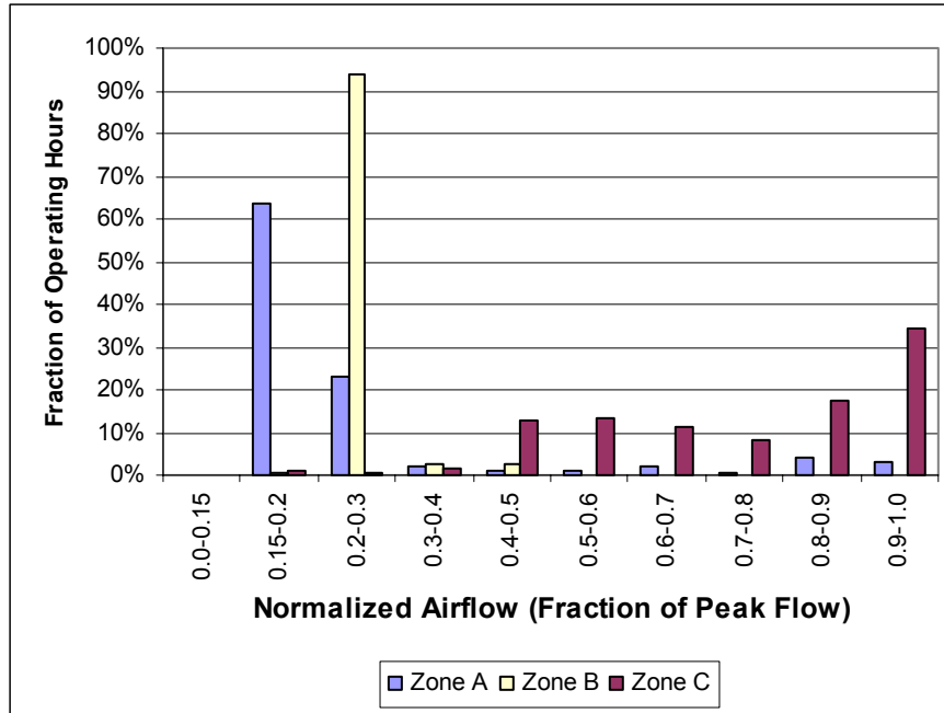
Figure 119. Site 4, Sample of Interior Zones (10/18/02-2/24/03)
