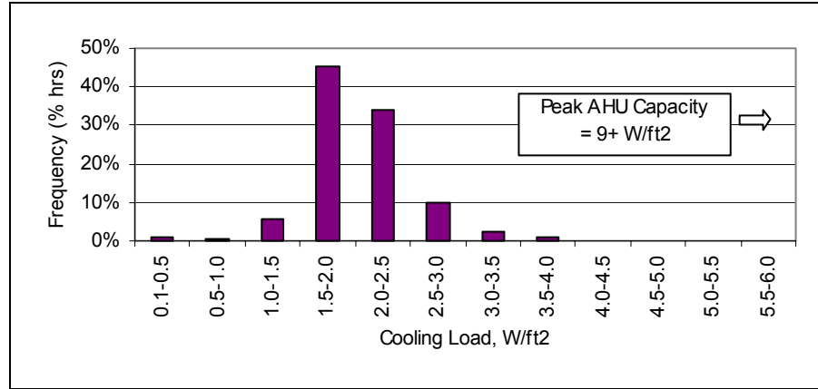
Figure 130. Site 4 (Dark bar includes Nov. 25, 2002 - Feb. 24, 2003)
