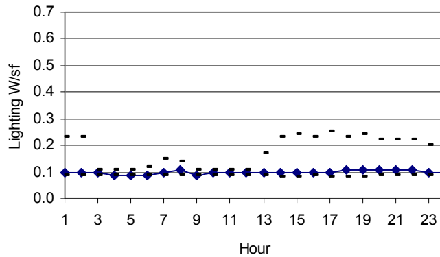
Figure 12. Measured Weekend Lighting Profile – Site 1 Office Area Showing Average (line) and Min/Max (dashes)
