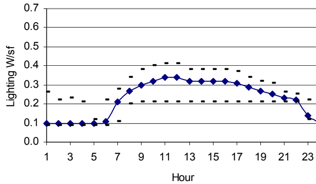
Figure 11. Measured Weekday Lighting Profile – Site 1 Office Area Showing Average (line) and Min/Max (dashes)
