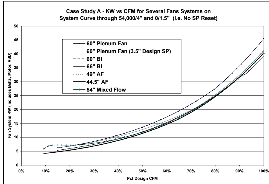
Figure 60. Case Study A - kW versus CFM
