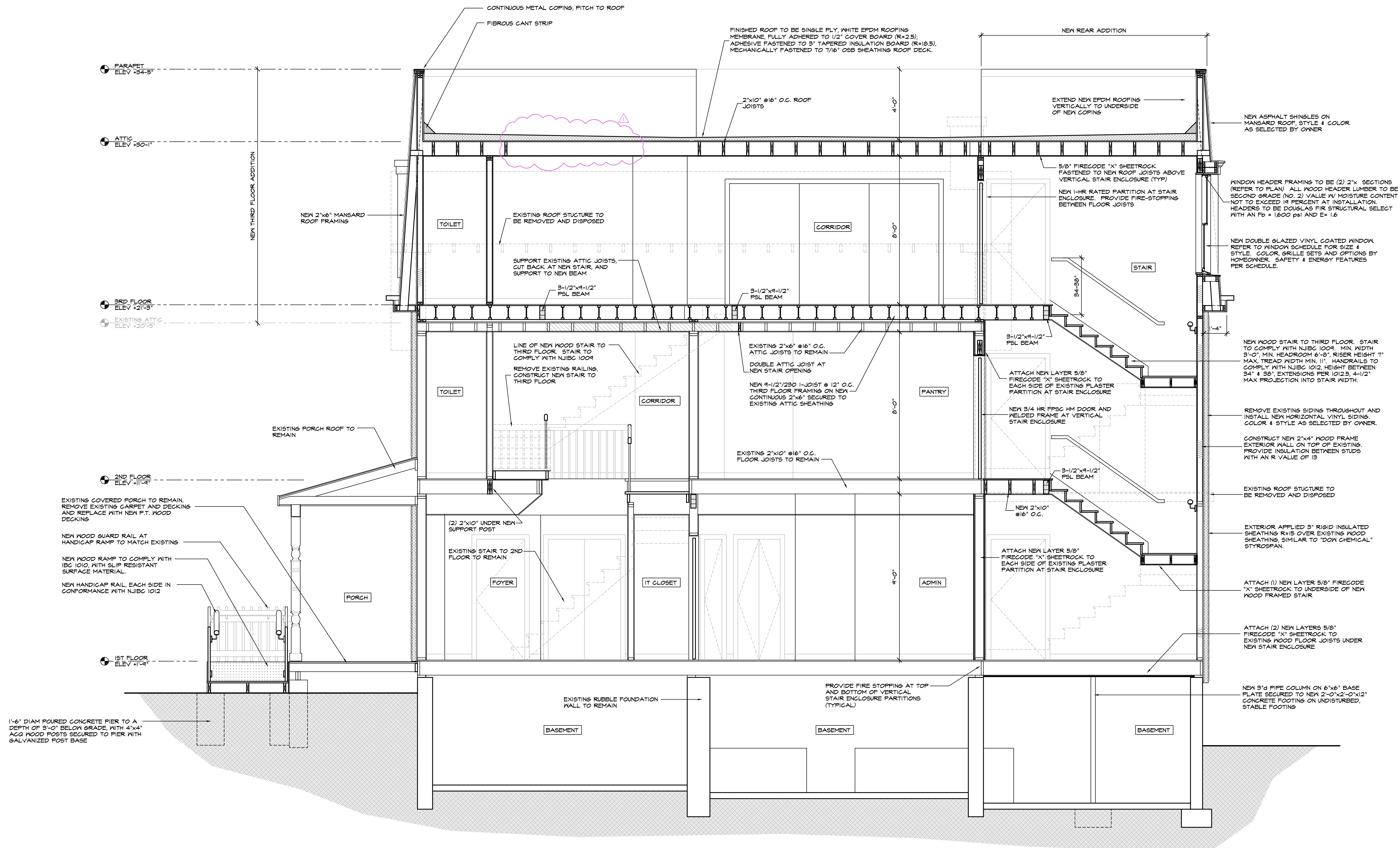
BUILDING CROSS SECTION "A-A"
